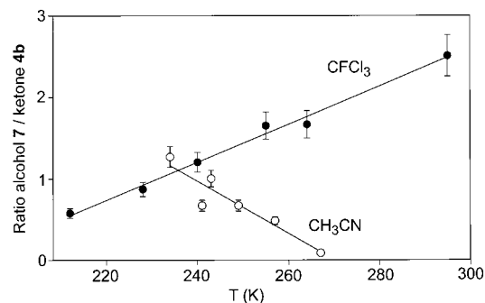
Figure 8. Ratio [alcohol 7 ]/[ketone 4b ] as a function of temperature and solvent. (○) acetonitrile; (●) CCl 3 F.
