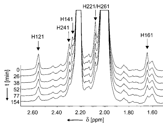
Figure 1. Aliphatic region of the 1 H NMR spectrum of 1b in CCl 3 F/(CBrF 2 ) at 233 K. Peaks marked by an arrow decrease with a first-order kinetics and are assigned to the methyl groups of 1b . The large peaks are due to unreacted diazo compound 2b .
